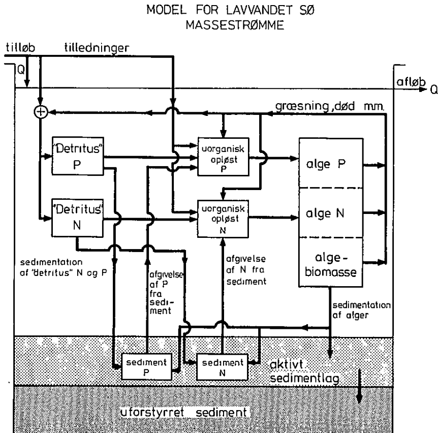
Figur 6.4 Blokdiagram for LAVSOE-modellen.
