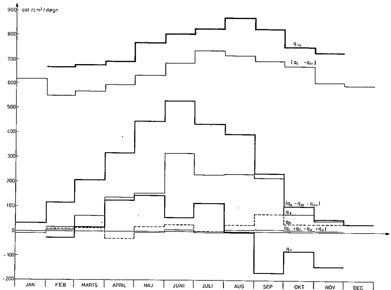
Figur 3.8 Extern-varmebalance, Mossø - 1975.
