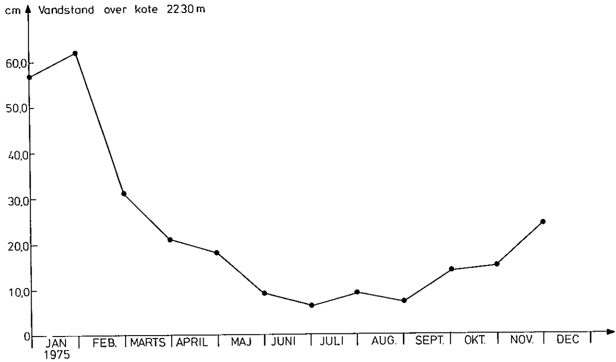
Figur 2.1 Vandstand, Mossø - 1975.
